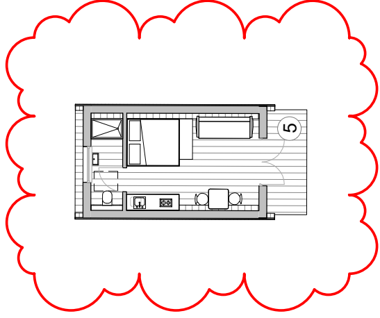
Cabin Floor Plan
